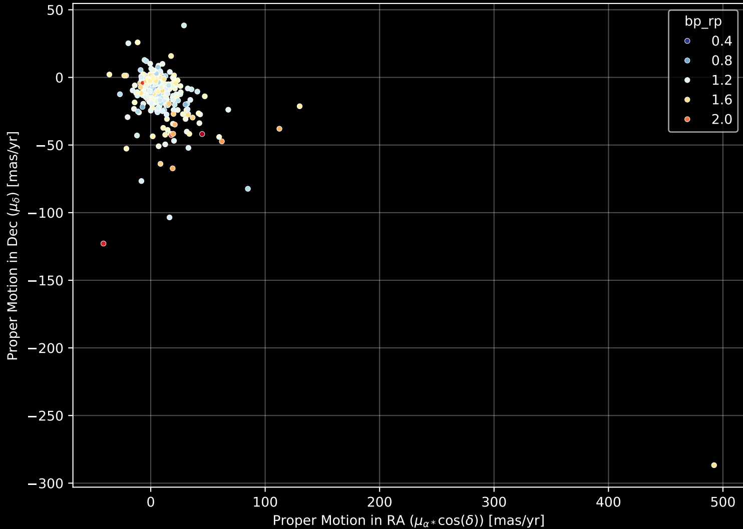
GALAH DR4 Field: [6585] Proper Motion Diagram (n= 457)
