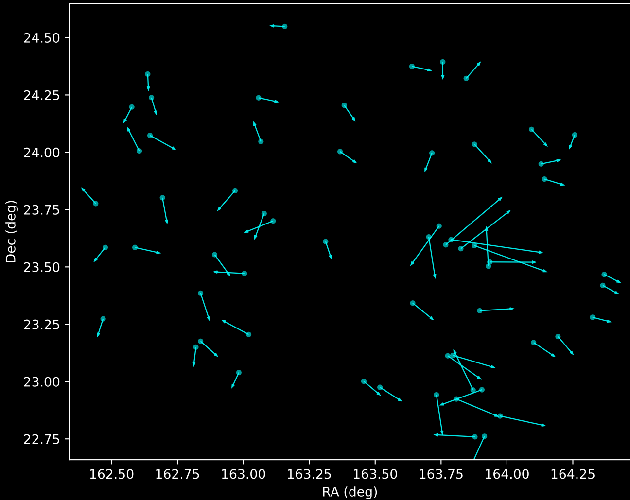
GALAH DR4 Noise Stream Proper Motion Vectors (n=61)
