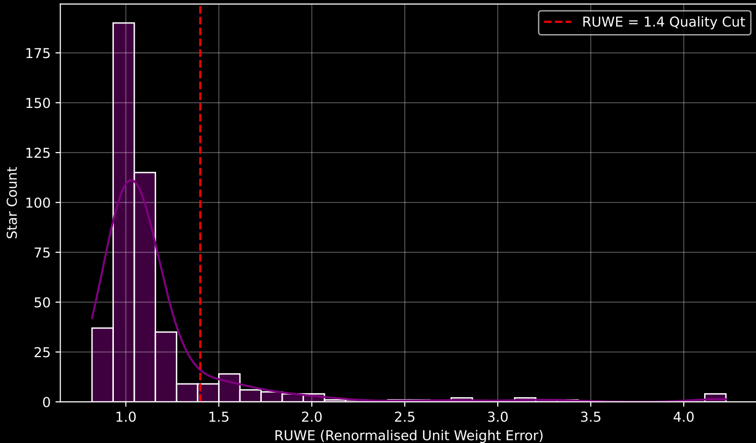
GALAH DR4 Field [6585] RUWE Distribution (n= 442)
