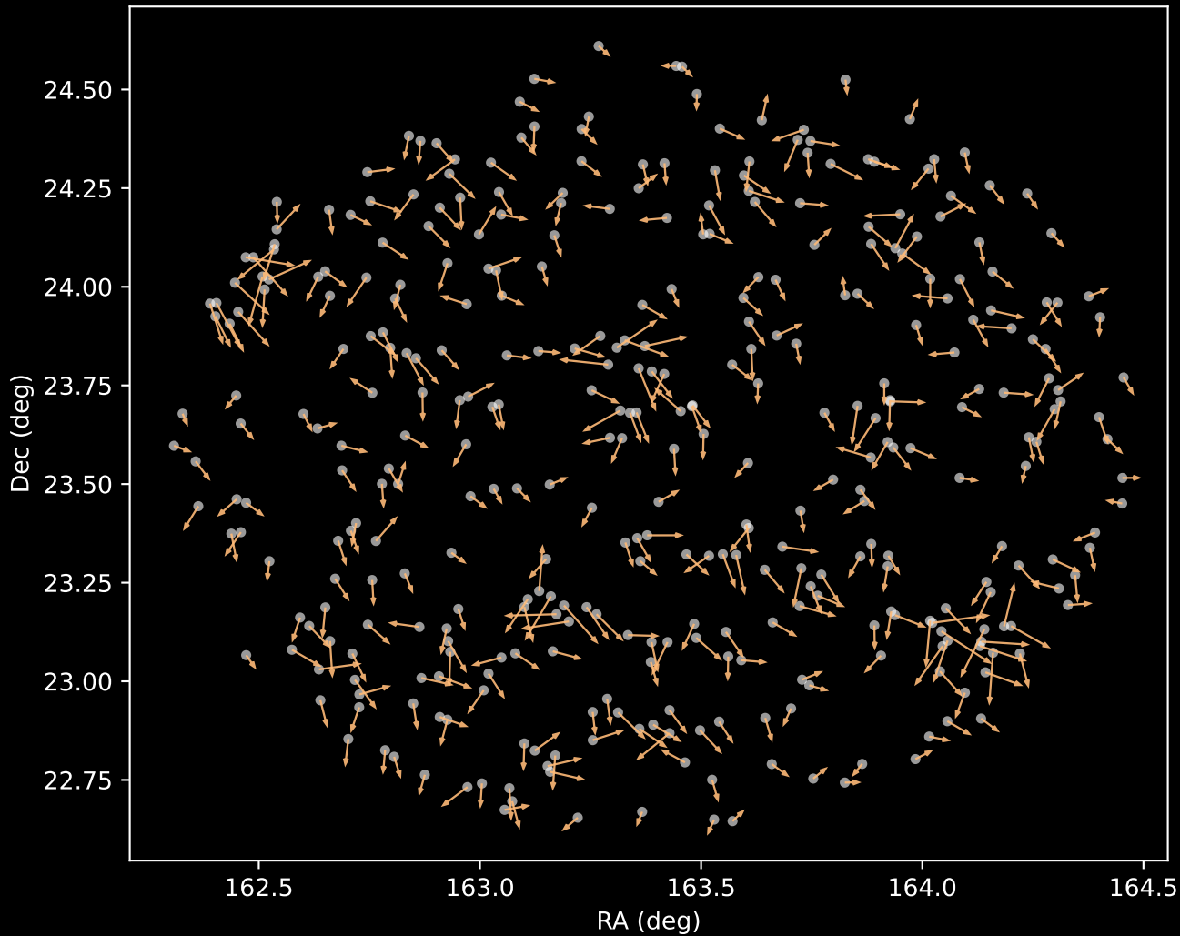
GALAH DR4 Cluster 3 Proper Motion Vectors (n=369)
