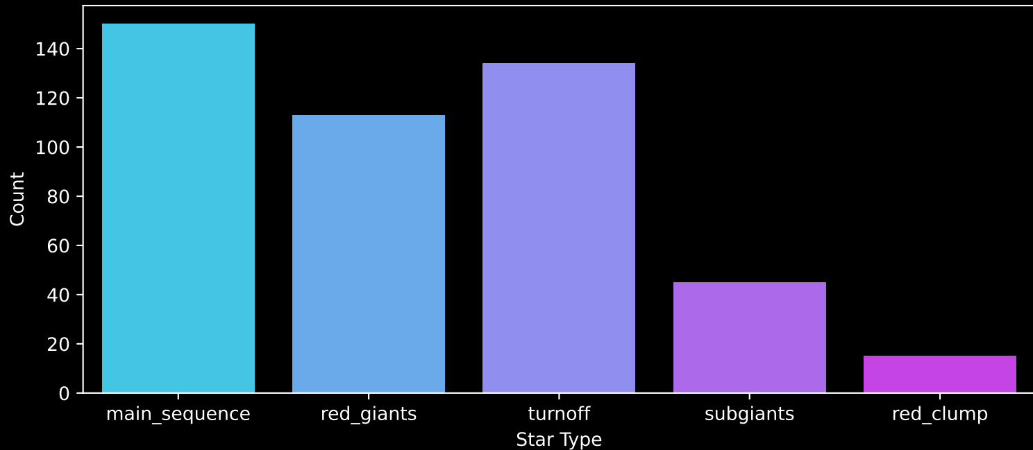
GALAH DR4 Field: [6585] Count plot of Star Type
